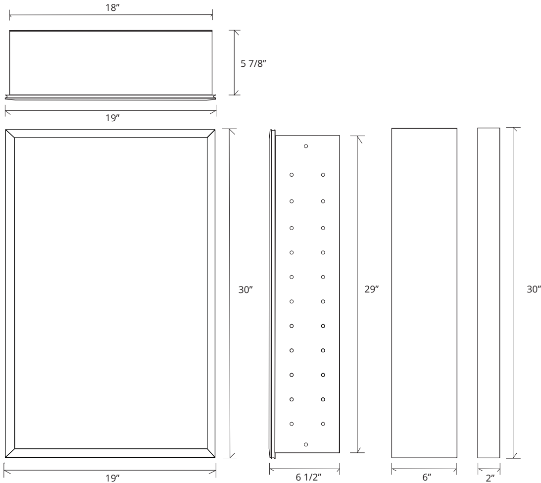
Beveled Mirror Section View
