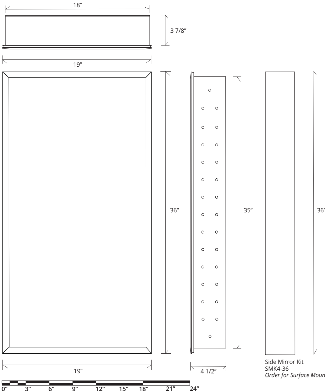
Beveled Mirror Section View
