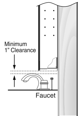
SURFACE MOUNT
