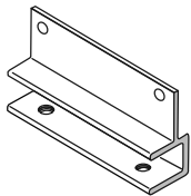
4" Clip Holder (2)
