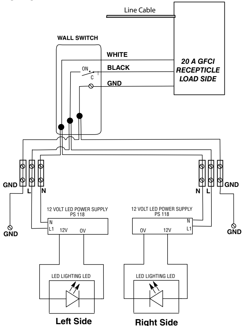
Wiring Diagram from a GFCI Outlet
