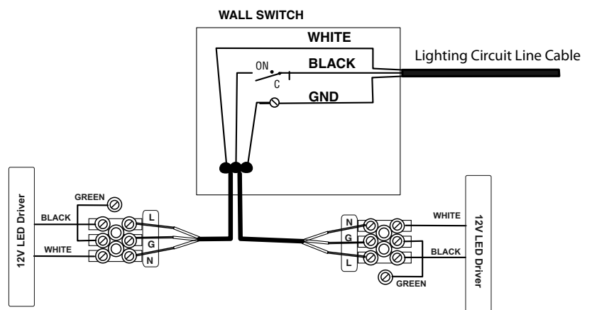
Alternate Wiring Diagram from a Switch
