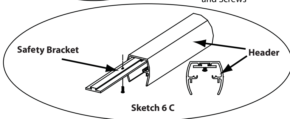
Anti-Lift Safety Brackets and Screws
